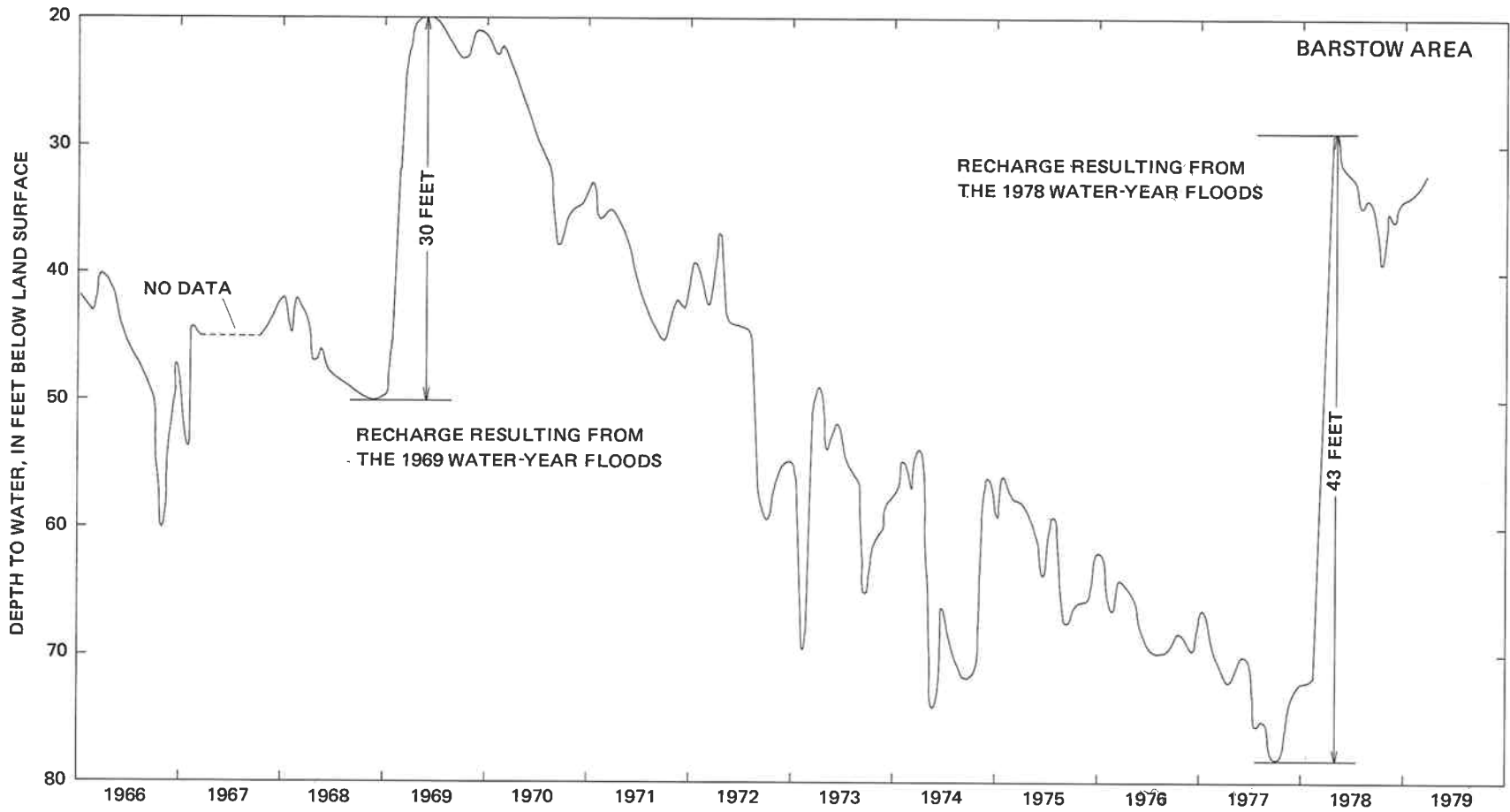
FIGURE 10.--Hydrograph of the Southern California Water Co. Arrowhead Plant well 4 (10N/1W-31L8) adjacent to the Mojave River in the middle basin. (Water-level data obtained from the Southern California Water Co., Los Angeles, Calif.)
