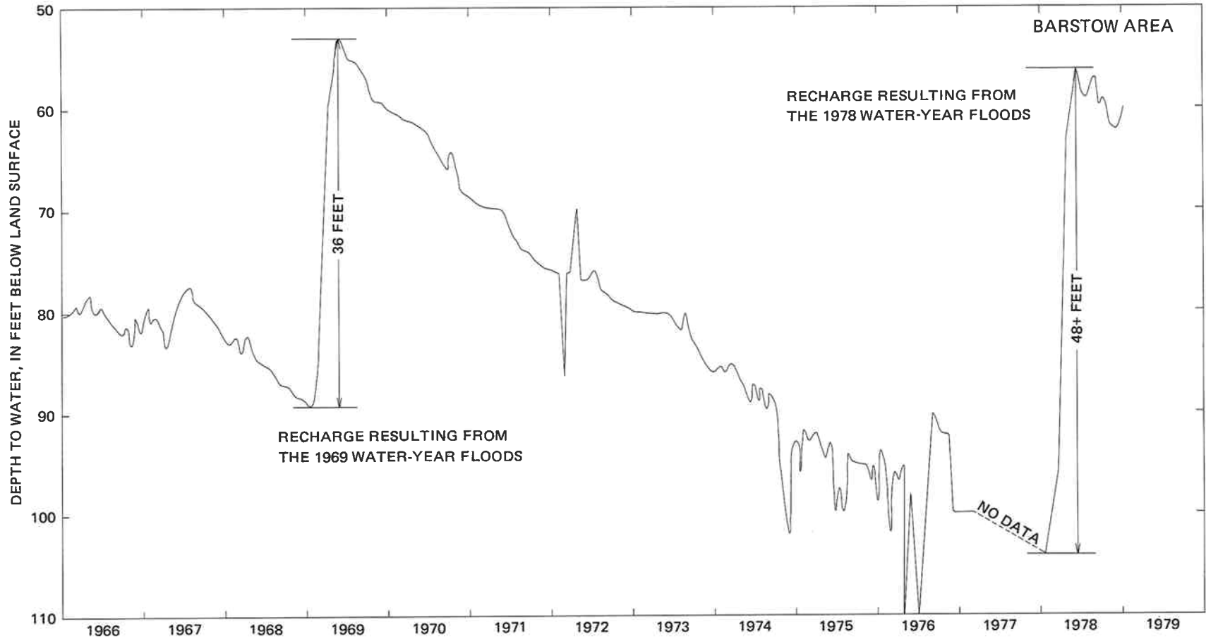
FIGURE 9.--Hydrograph of the Southern California Water Co. Robinson Plant well 16 (9N/2W-10A2) adjacent to the Mojave River in the middle basin. (Water-level data obtained from the Southern California Water Co., Los Angeles, Calif.)
