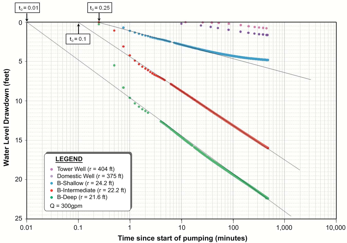
Figure 31 Time-Drawdown Plot for Cluster B, Domestic, and Tower Observation Wells
